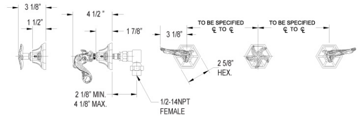
DIVERTER HANDLE HOT & COLD HANDLE
