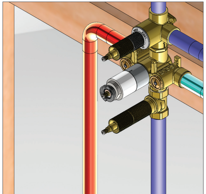
Fully installed Extension Kit
