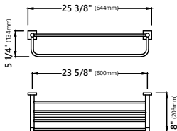
Model #: KEA-17742 Shelf with Towel Bar Dimensions: 25 3/8" x 8" x 5 1/4"
