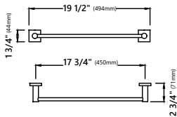
Model #: KEA-17736 Towel Bar Dimensions: 19 1/2" x 2 3/4" x 1 3/4"
