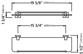
Model #: KEA-17745 Bathroom Shelf Dimensions: 19 5/8" x 5 1/2" x 1 3/4"
