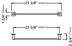
Model #: KEA-17737 Towel Bar Dimensions: 25 3/8" x 2 3/4" x 1 3/4"
